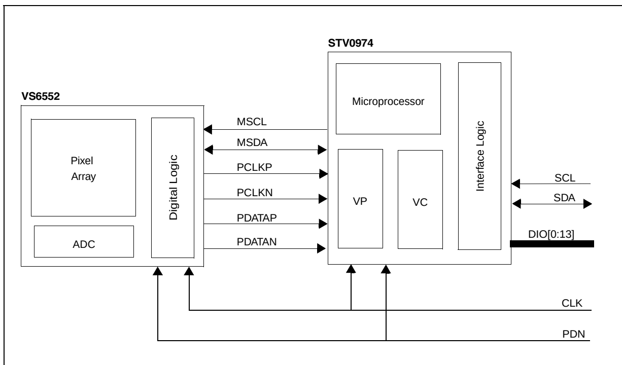
Figure 1. Camera System Using STV0974
